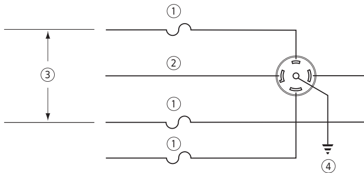
Figure 1.2 Three-Phase “Y” Electrical Requirements
