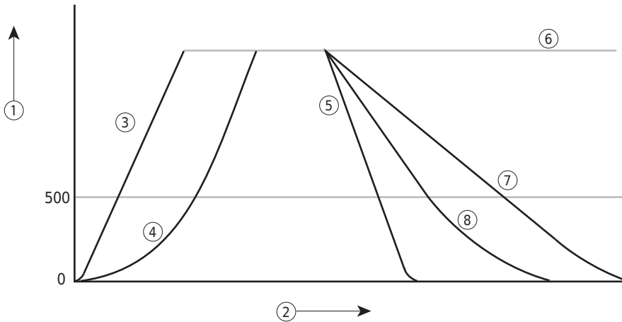
Figure 3.1 Acceleration and Deceleration Settings Graph
