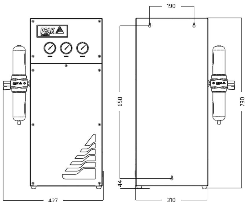
Infinity 1032 & 1033 in mm
