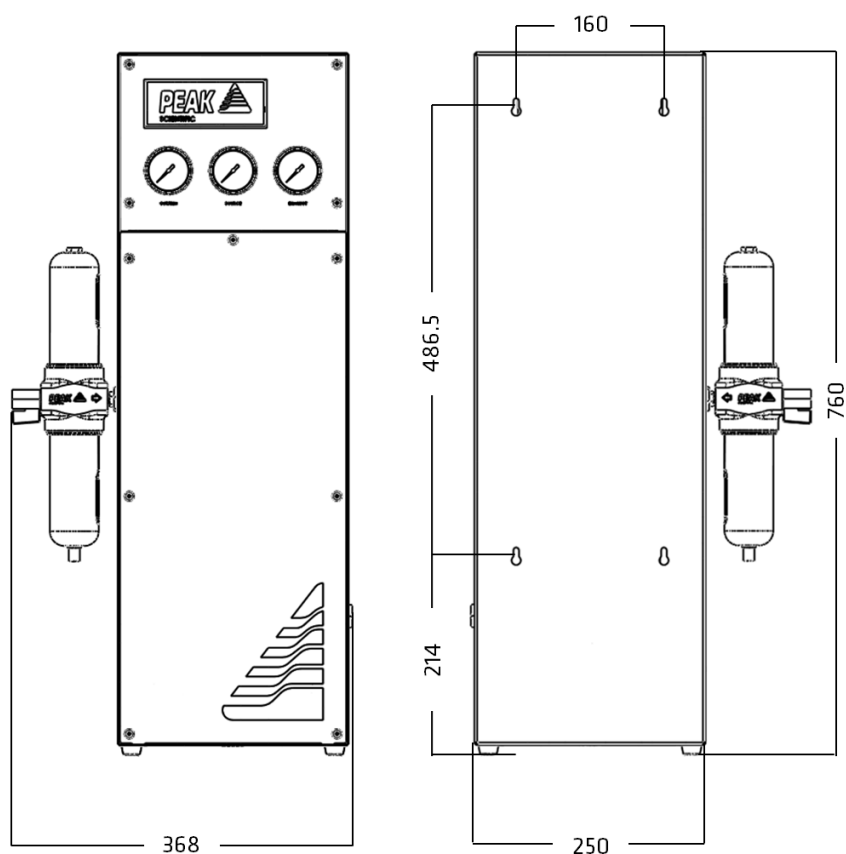
Infinity 1031/Hi-Flow in mm
