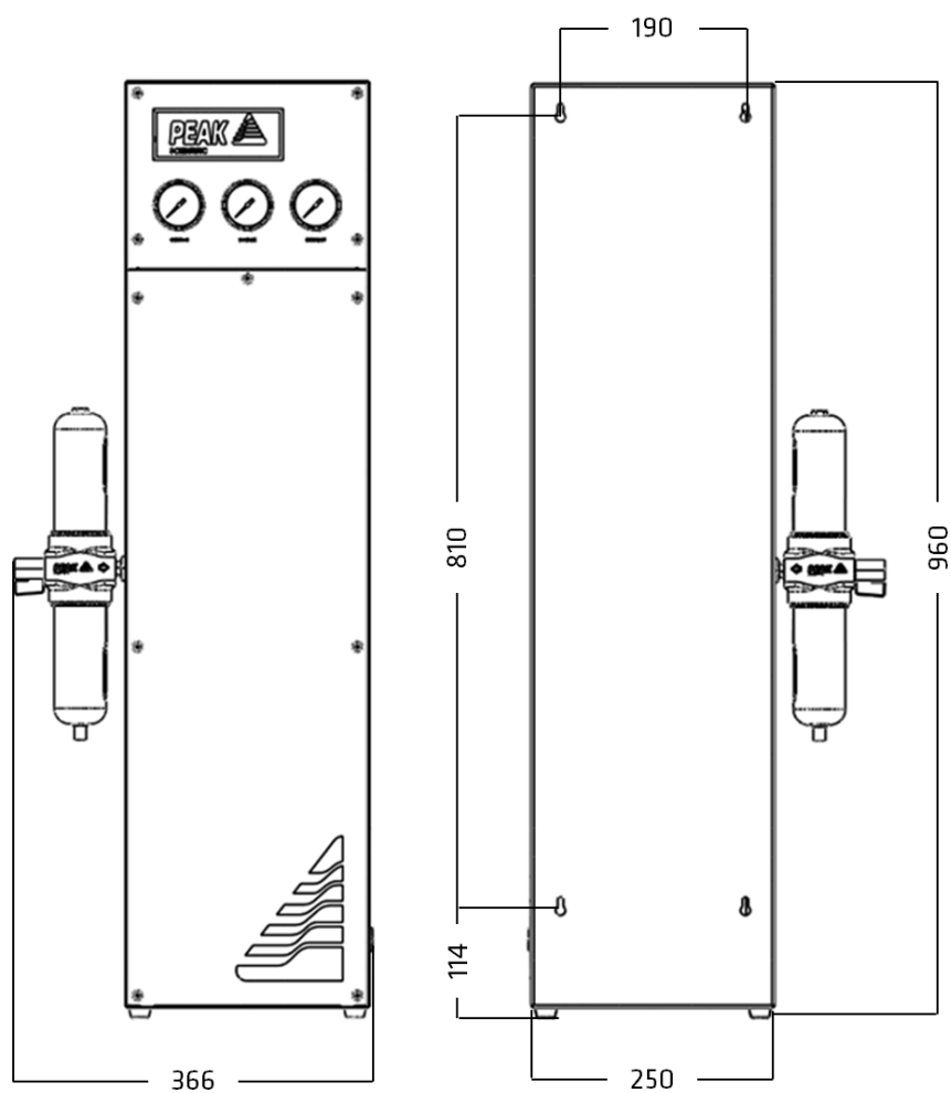
Infinity 1034 in mm
